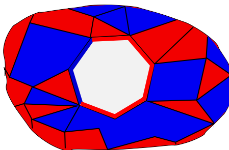
Figure 2: Example of surface generated by \langle \text{Tr } M_1^2 M_2^5 \rangle_c : it is a disc with one boundary of length 7 with red condition for 5 adjacent segments followed by two segments with blue condition.
